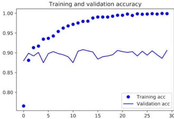
Figure 5.15 Training and validation accuracy for simple feature extraction
