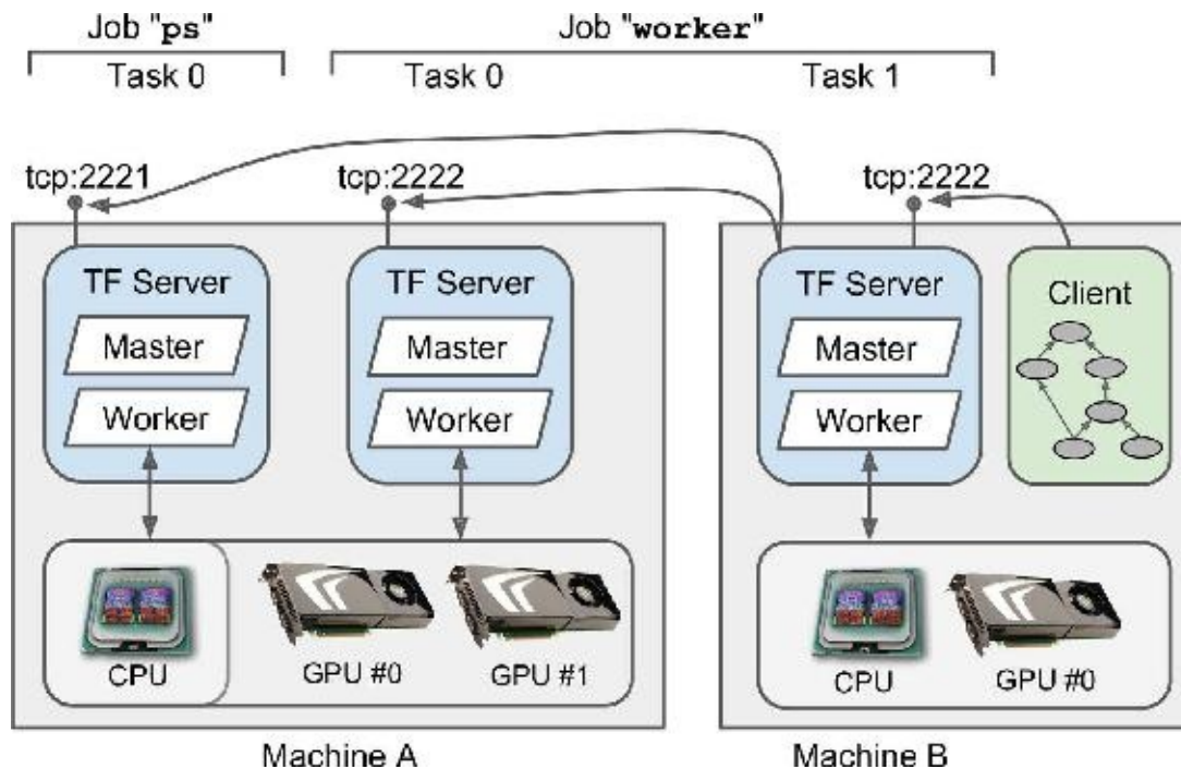
Figure 12-6. TensorFlow cluster
