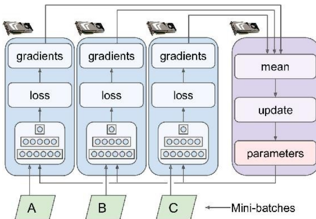
Figure 12-17. Data parallelism
