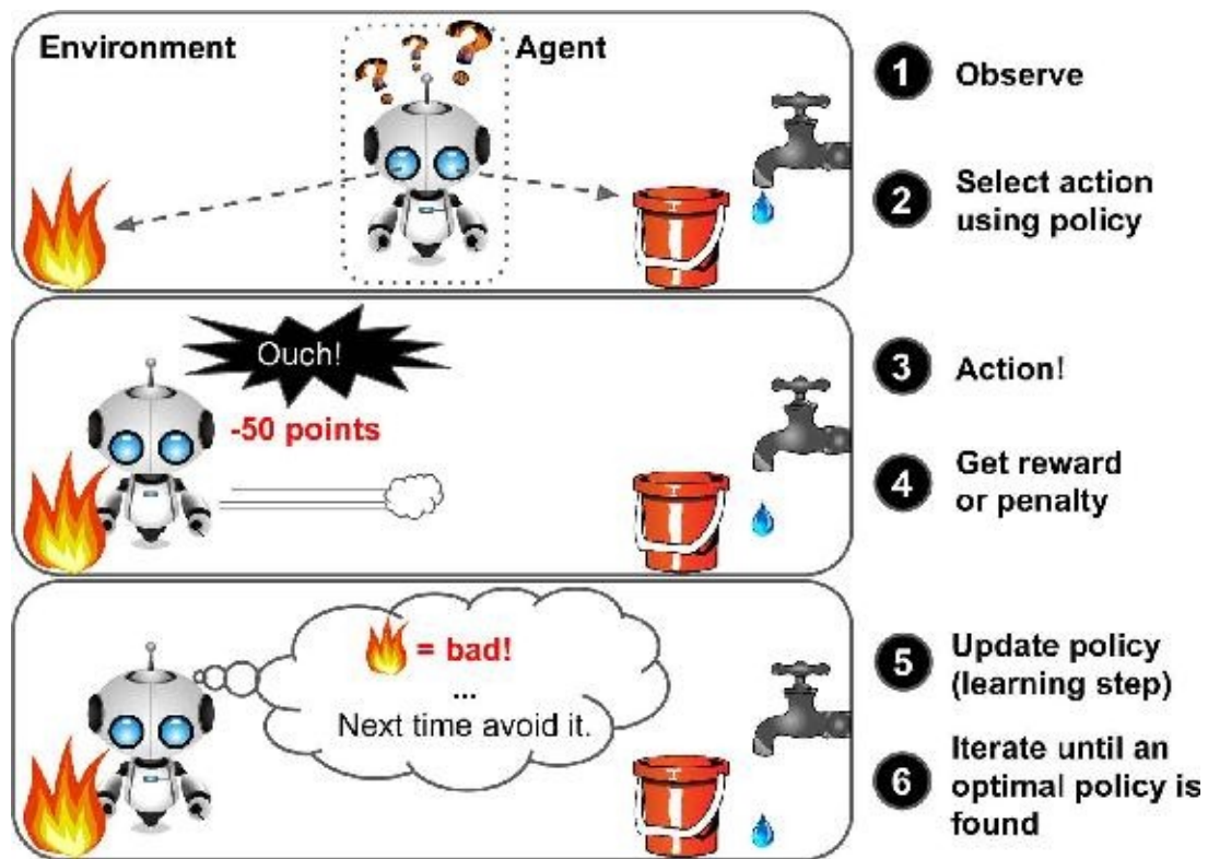
Figure 1-12. Reinforcement Learning
