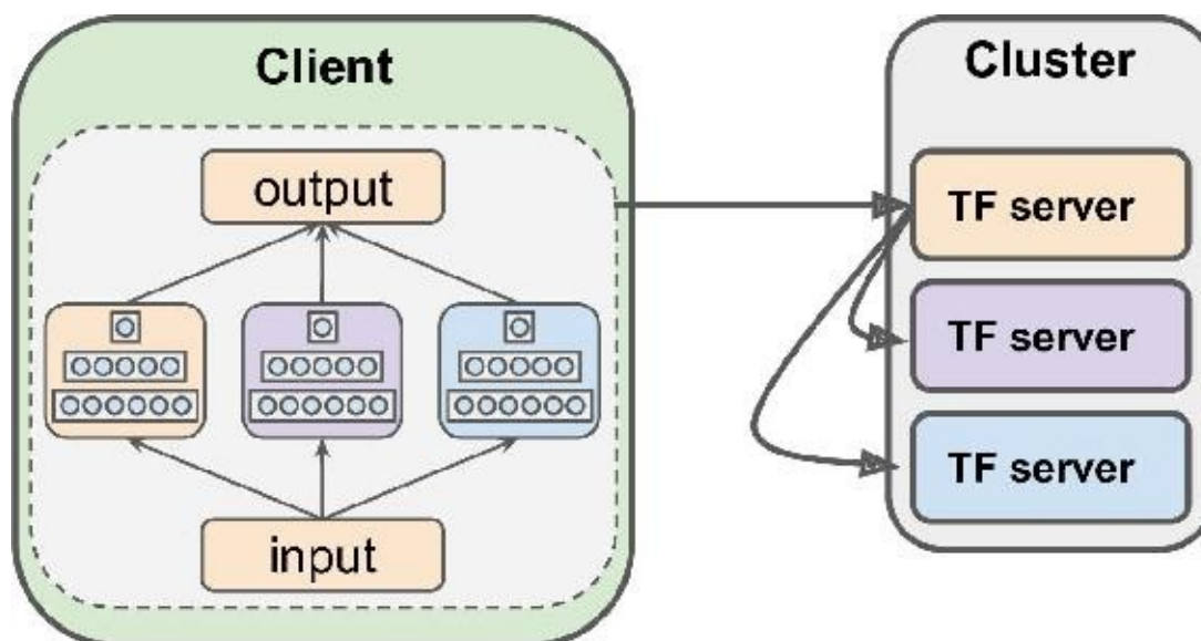
Figure 12-12. In-graph replication
