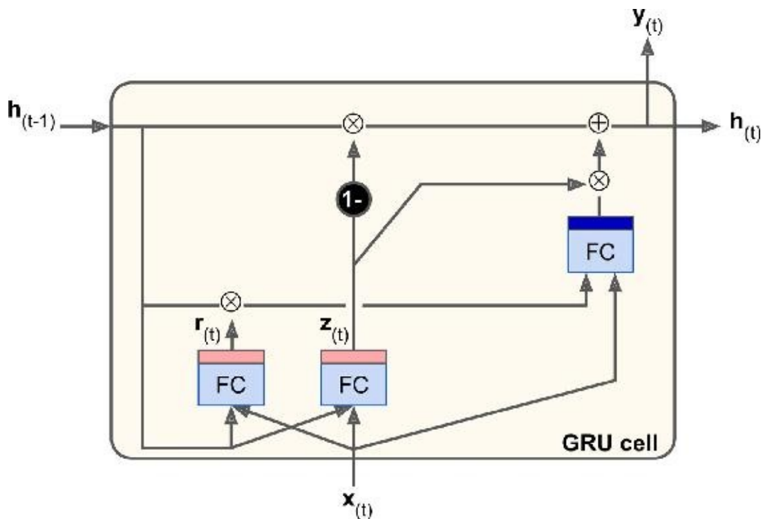
Figure 14-14. GRU cell
