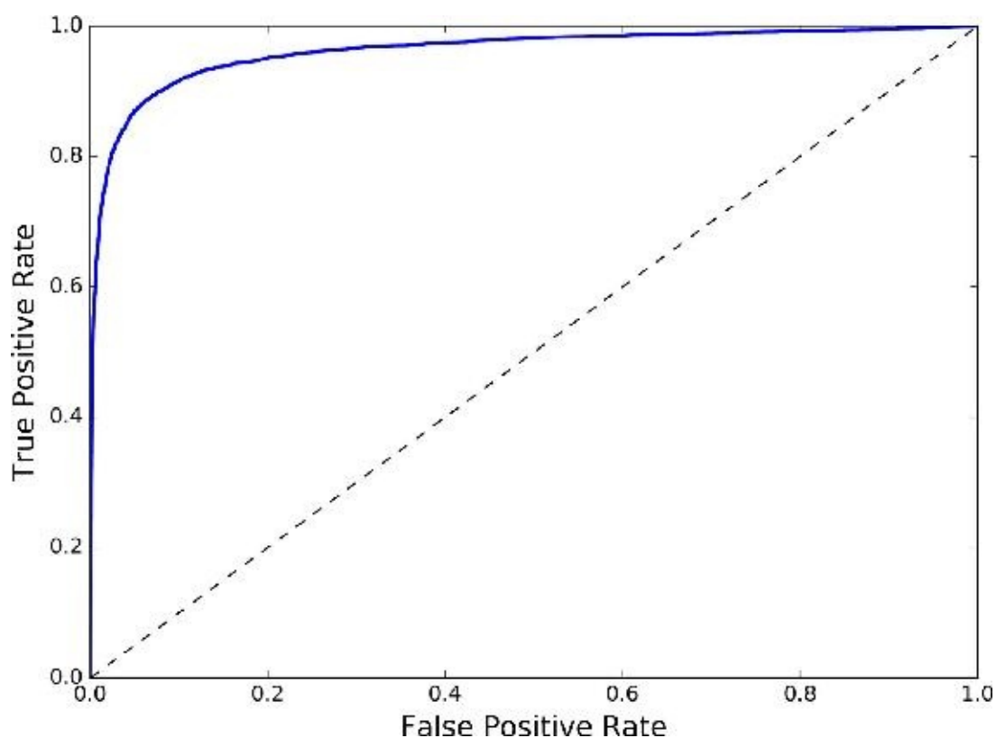
Figure 3-6. ROC curve
