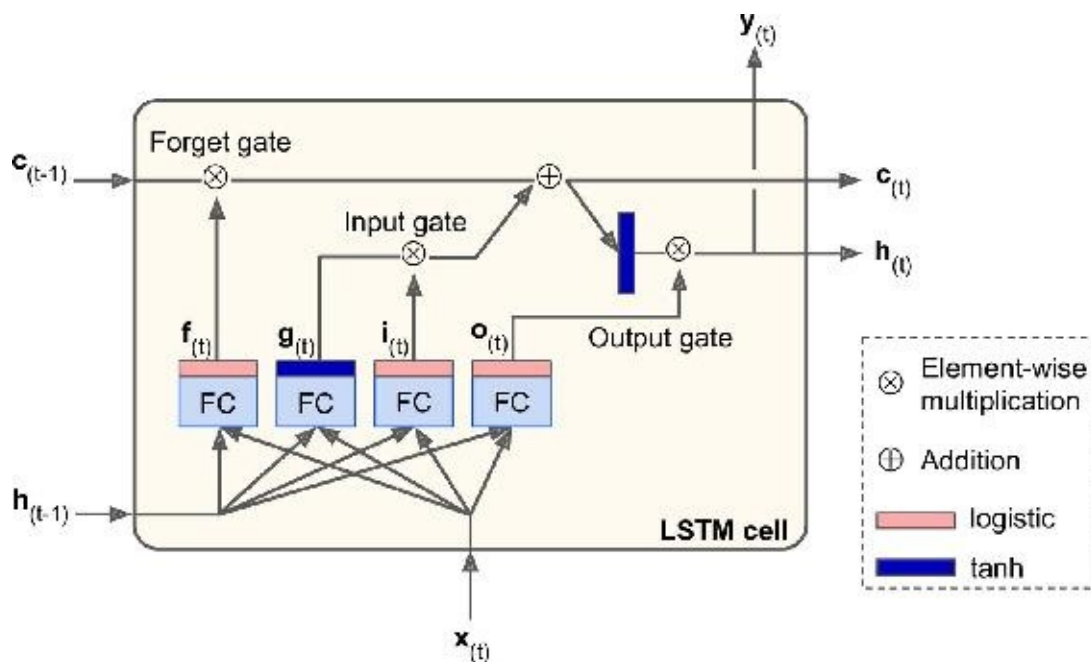
Figure 14-13. LSTM cell
