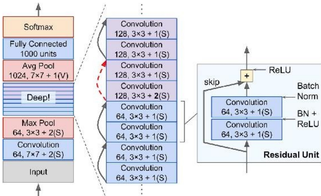
Figure 13-14. ResNet architecture
