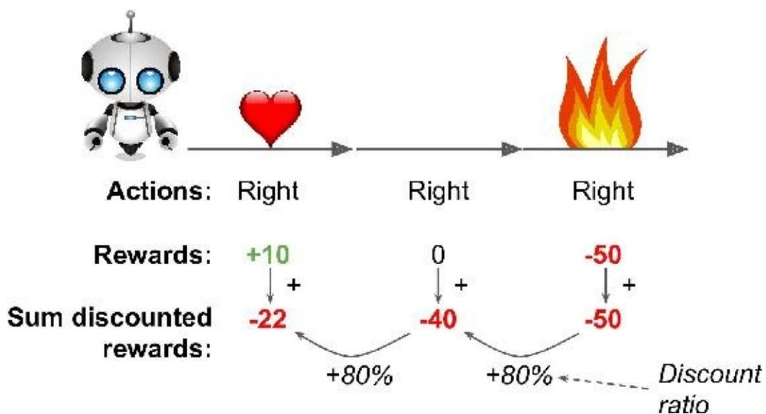
Figure 16-6. Discounted rewards
