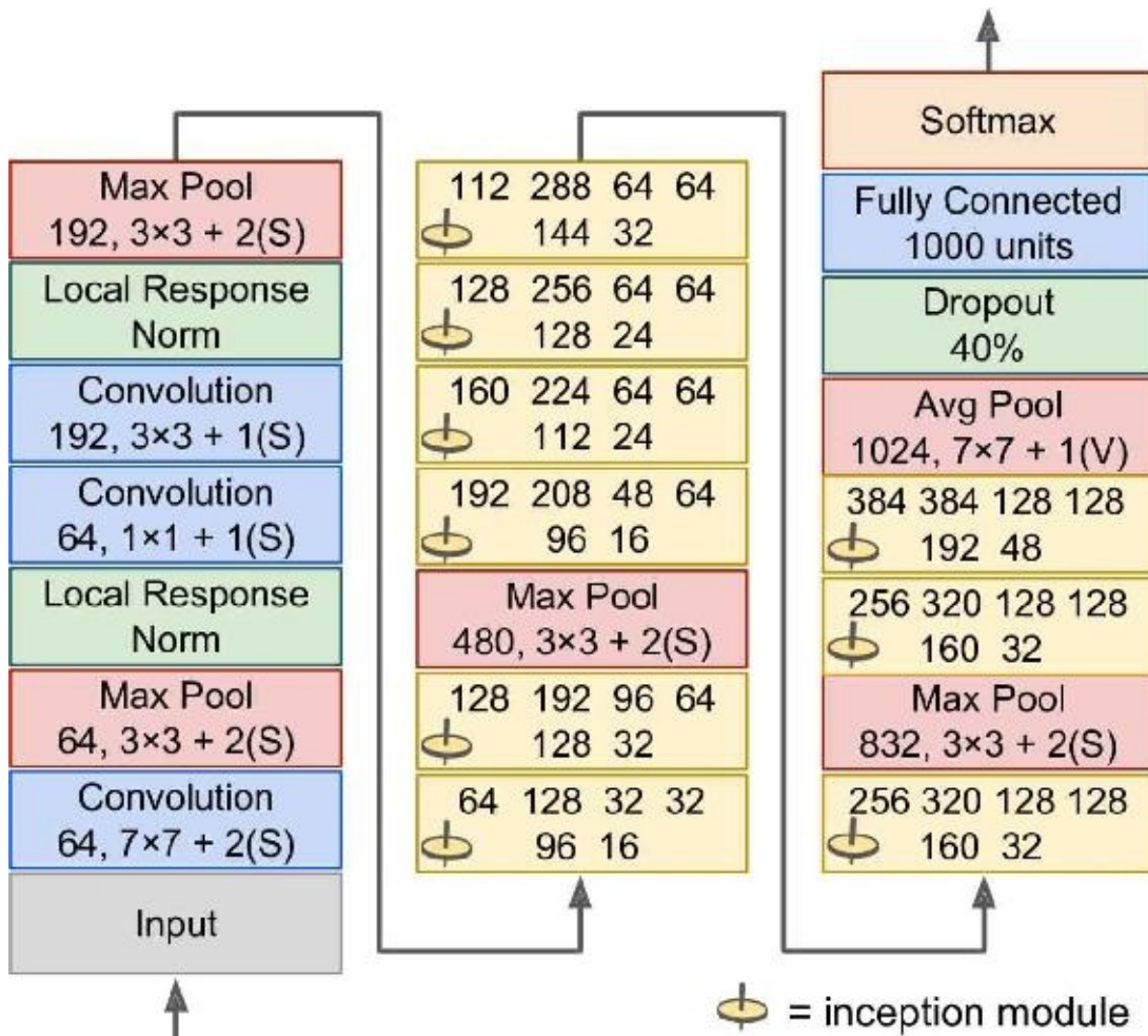
Figure 13-11. GoogLeNet architecture
