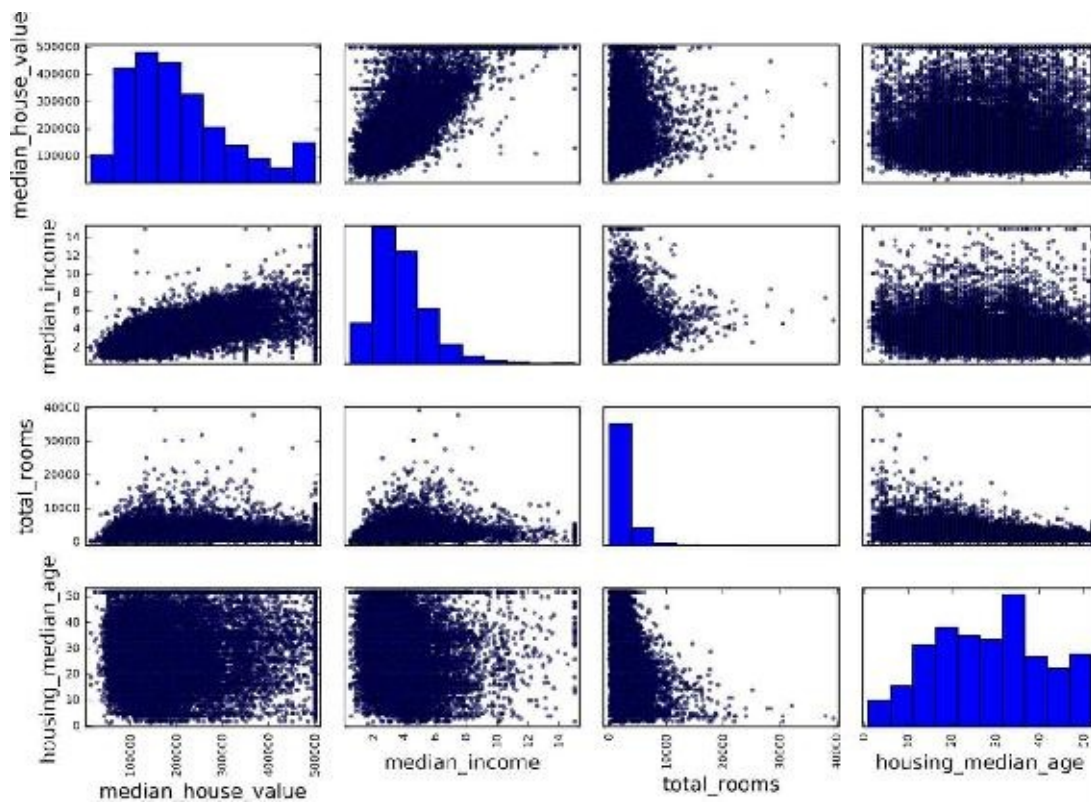
Figure 2-15. Scatter matrix
