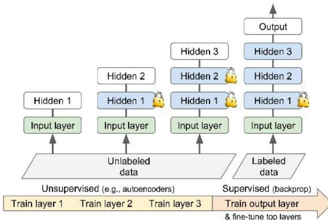
Figure 11-5. Unsupervised pretraining
