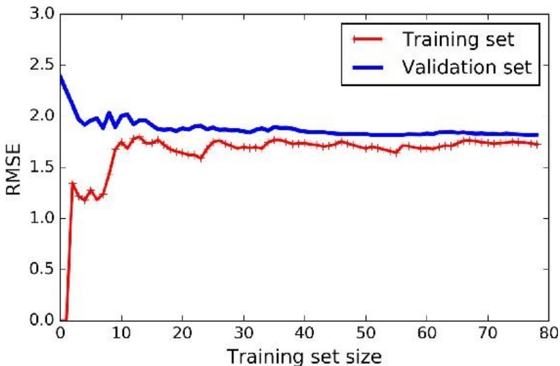
Figure 4-15. Learning curves
