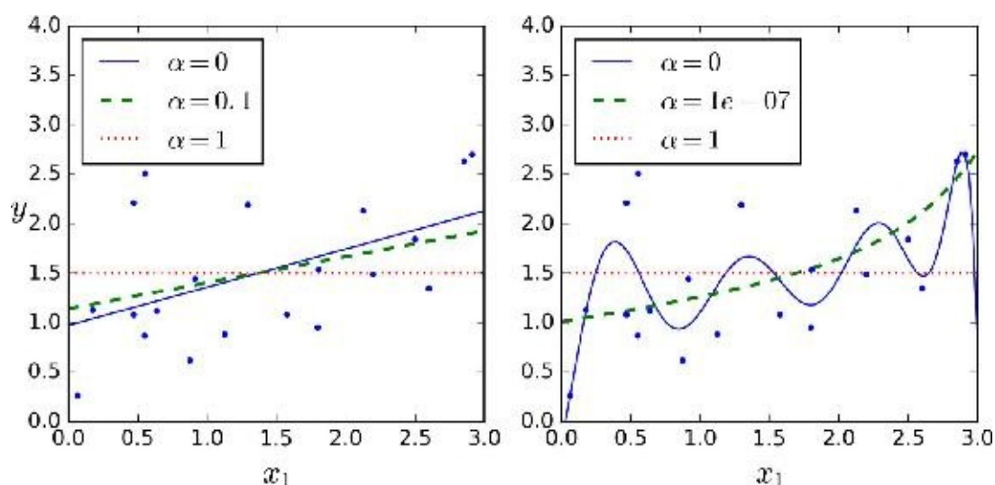
Figure 4-18. Lasso Regression
