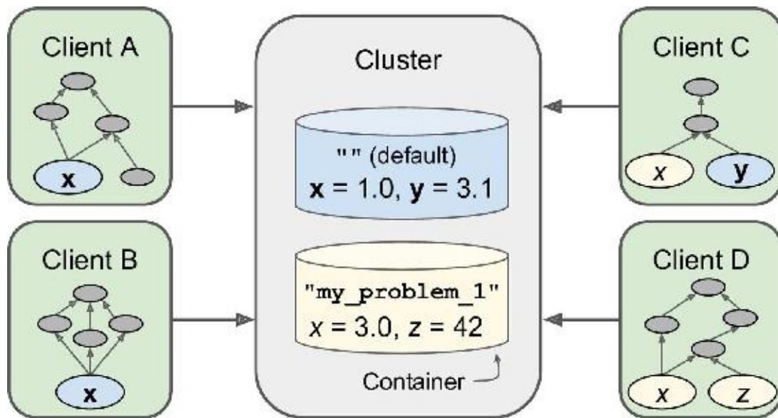
Figure 12-7. Resource containers
