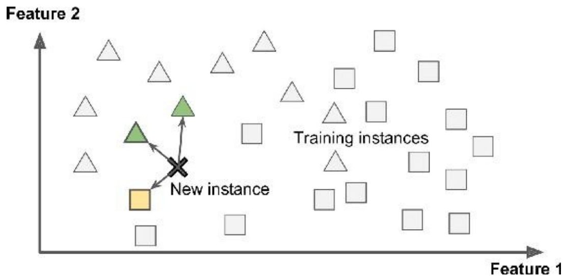
Figure 1-15. Instance-based learning
