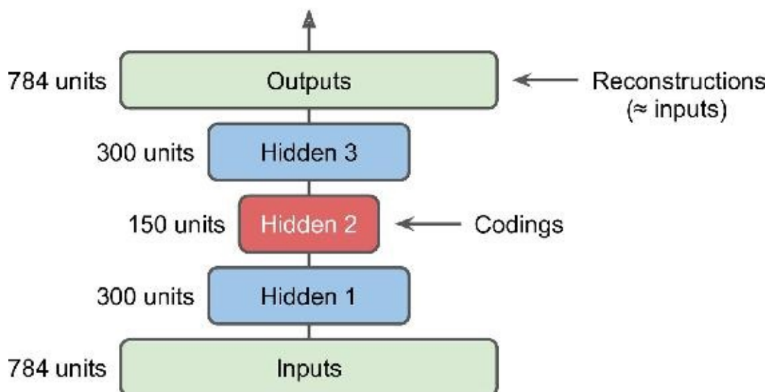
Figure 15-3. Stacked autoencoder
