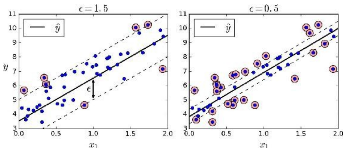
Figure 5-10. SVM Regression
