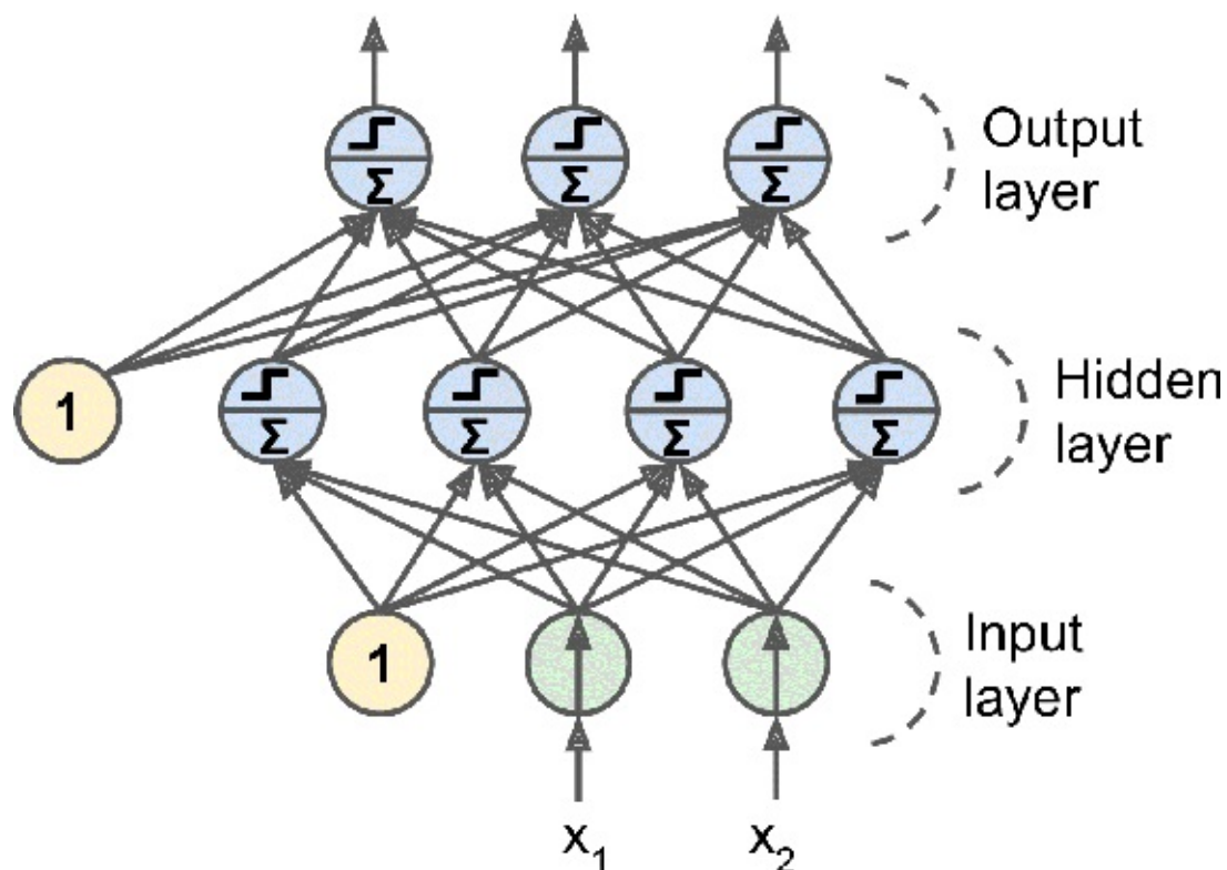
Figure 10-7. Multi-Layer Perceptron
