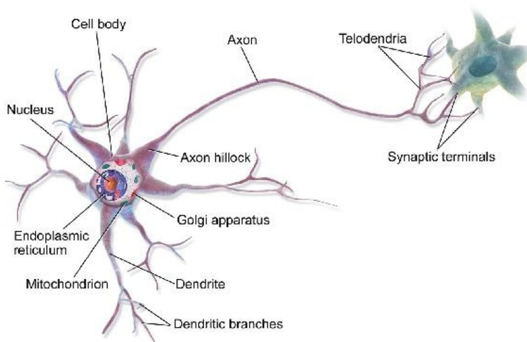
Figure 10-1. Biological neuron 3
