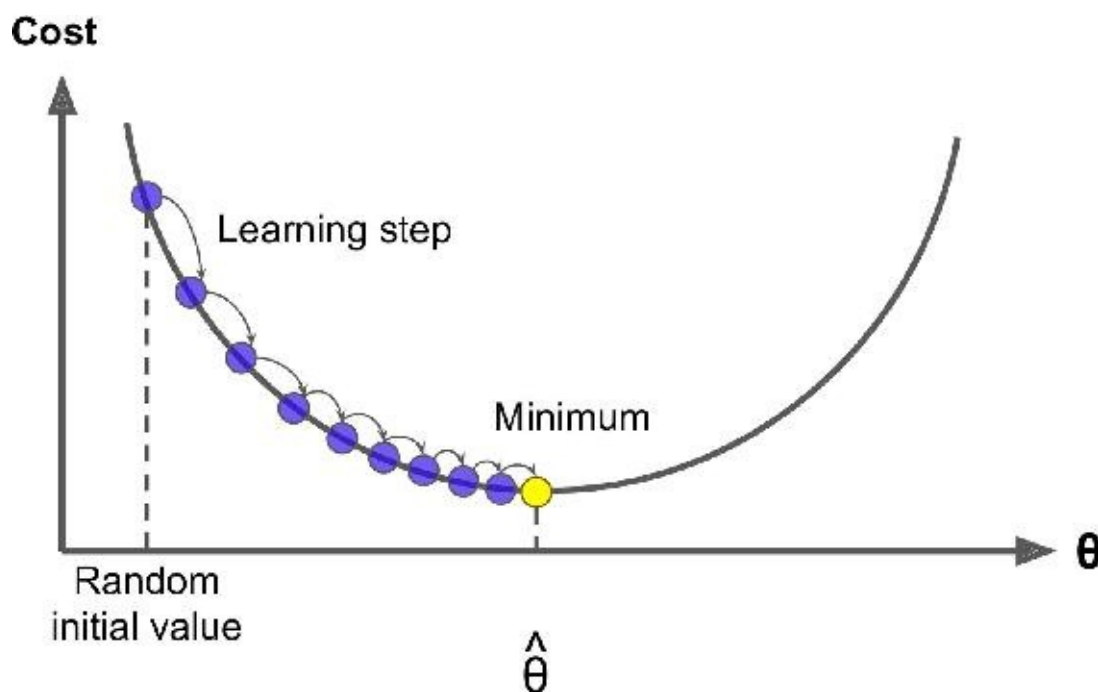
Figure 4-3. Gradient Descent
