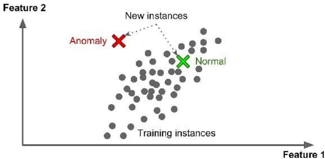
Figure 1-10. Anomaly detection
