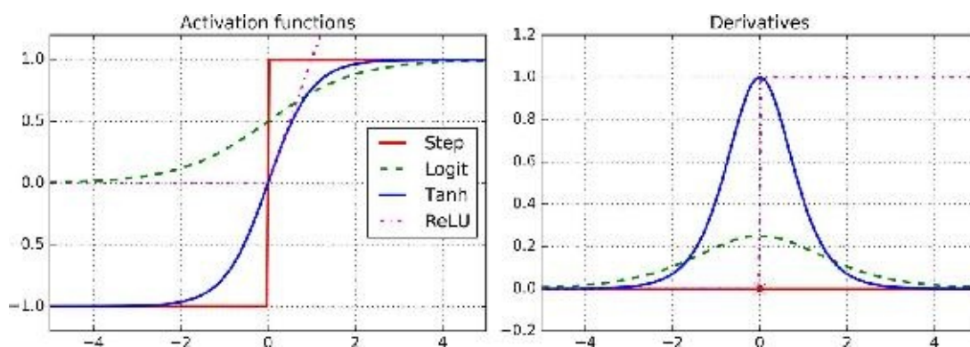
Figure 10-8. Activation functions and their derivatives
