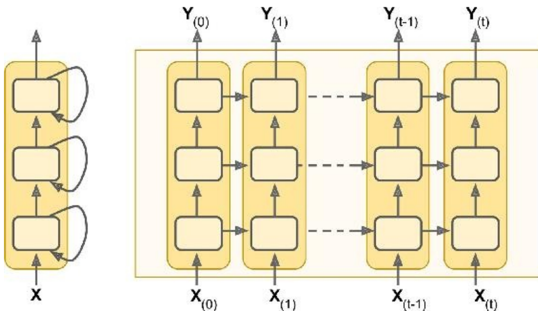
Figure 14-12. Deep RNN (left), unrolled through time (right)
