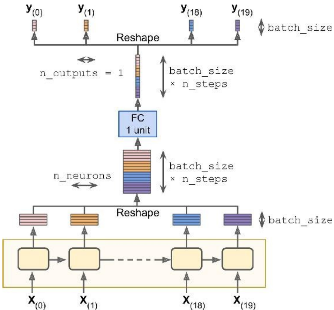
Figure 14-10. Stack all the outputs, apply the projection, then unstack the result
