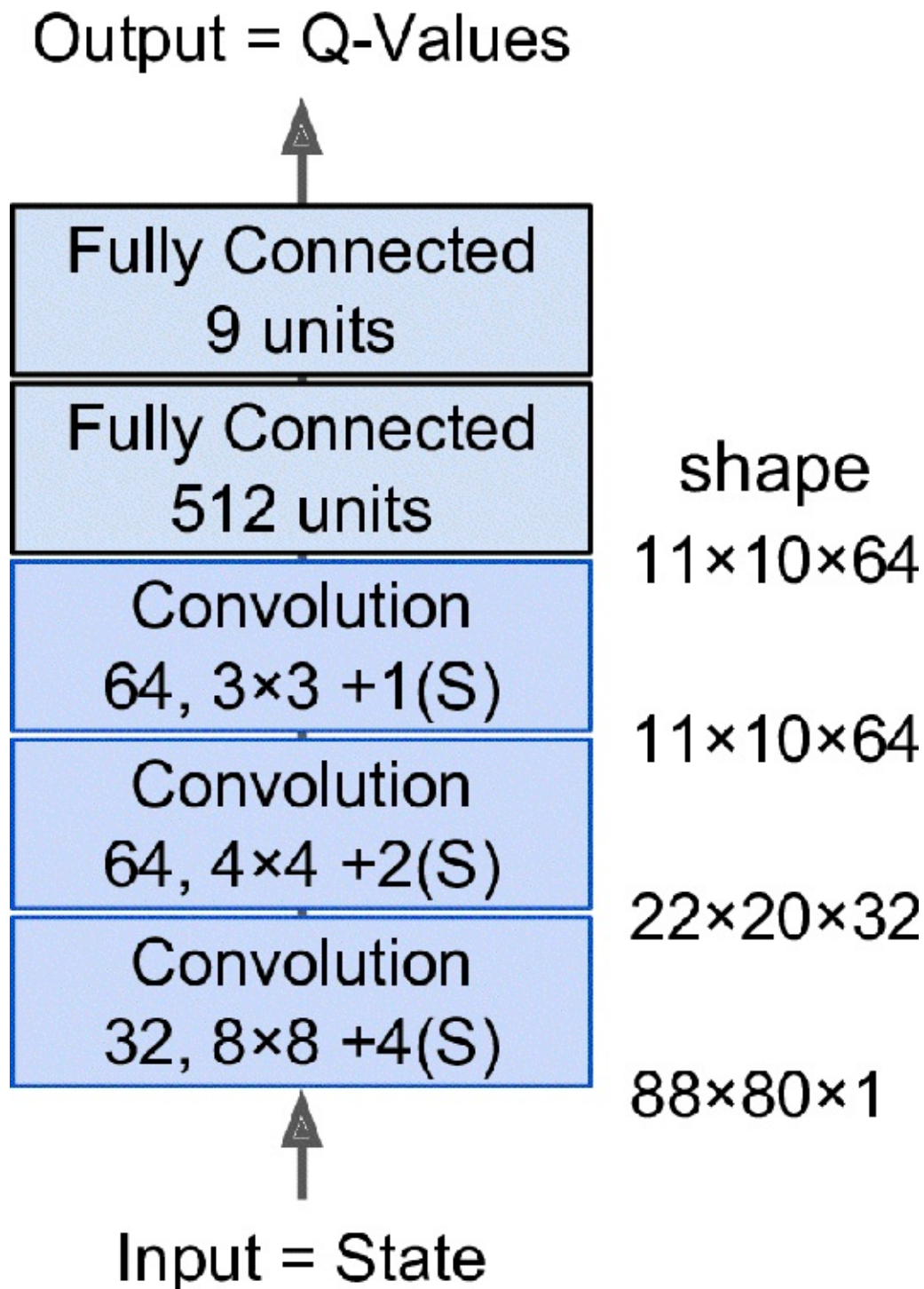
Figure 16-10. Deep Q-network to play Ms. Pac-Man
