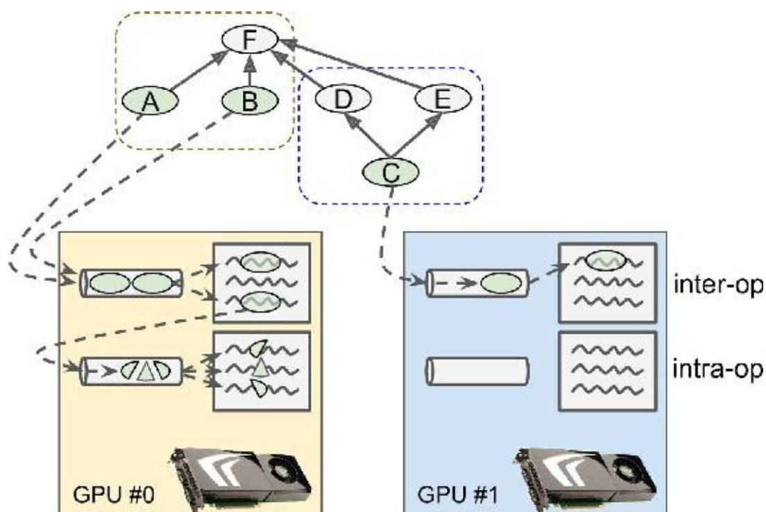
Figure 12-5. Parallelized execution of a TensorFlow graph
