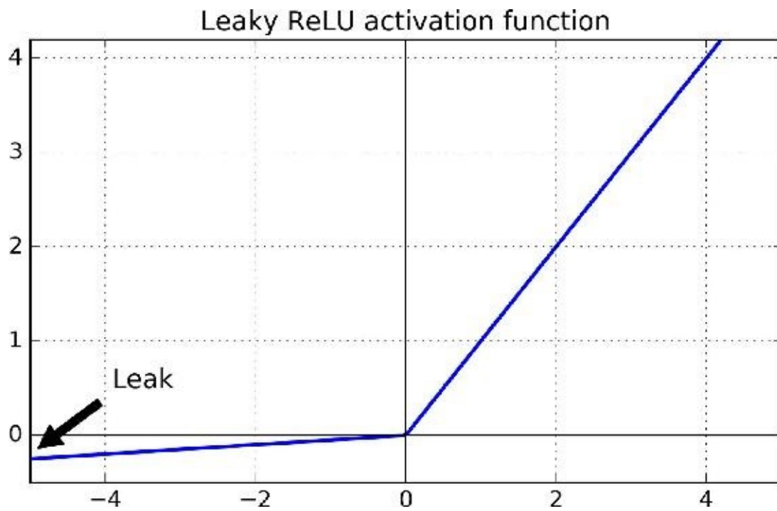
Figure 11-2. Leaky ReLU
