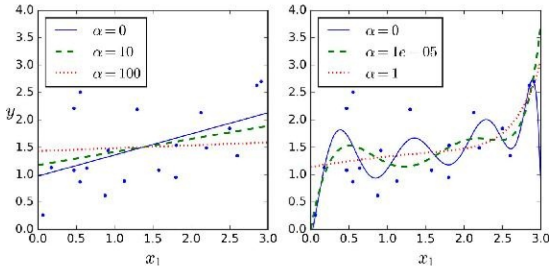
Figure 4-17. Ridge Regression
