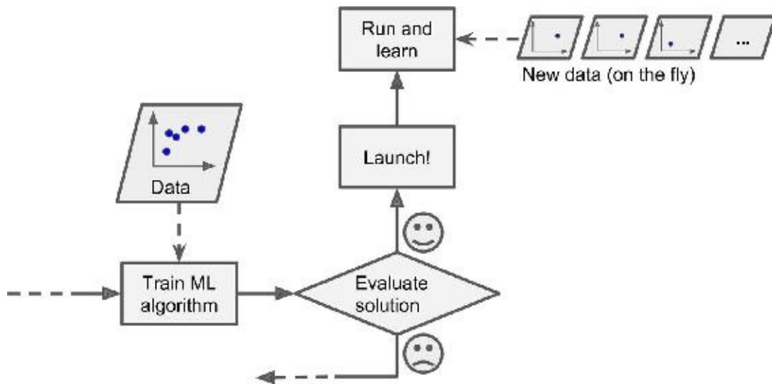
Figure 1-13. Online learning
