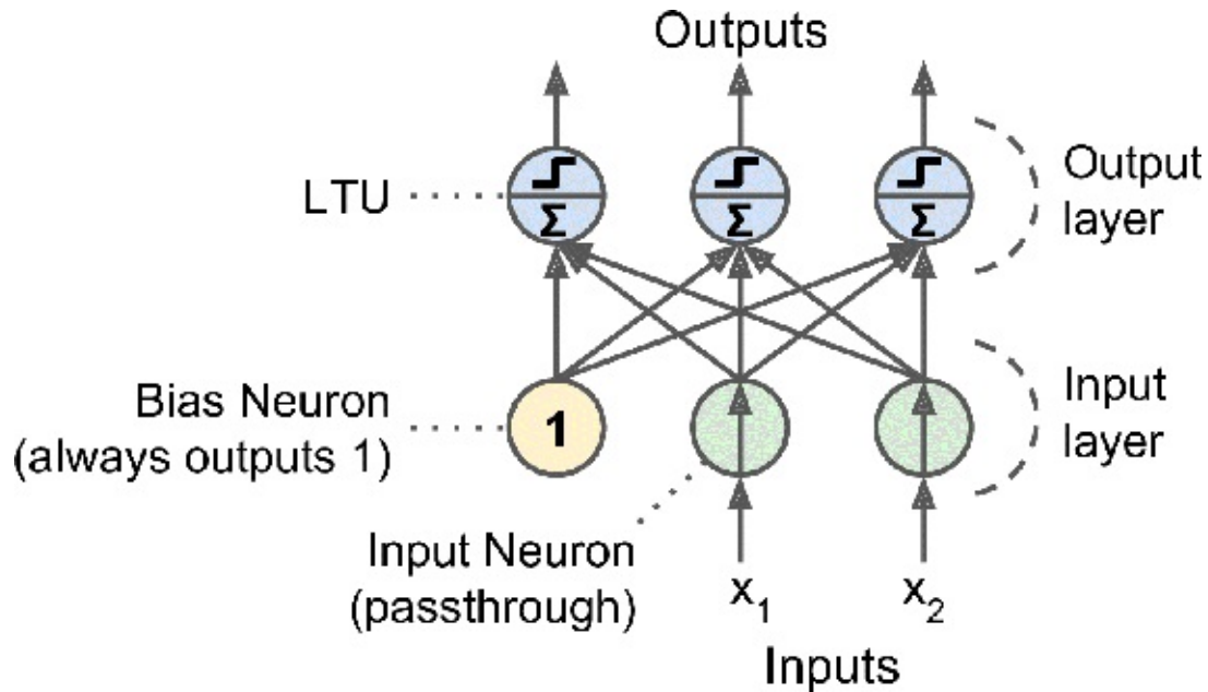
Figure 10-5. Perceptron diagram
