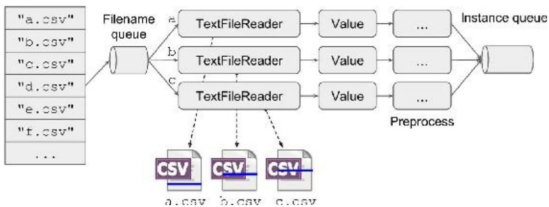
Figure 12-10. Reading simultaneously from multiple files
