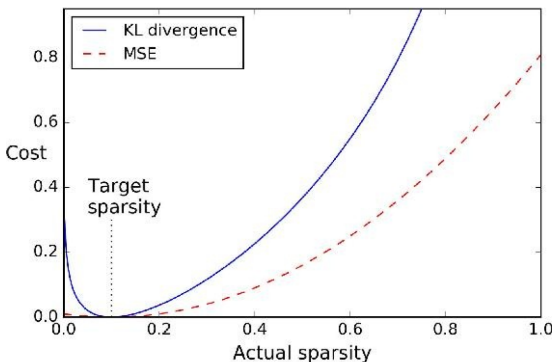
Figure 15-10. Sparsity loss
