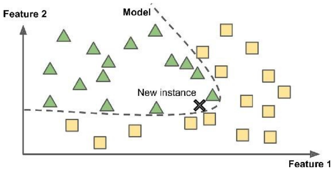
Figure 1-16. Model-based learning
