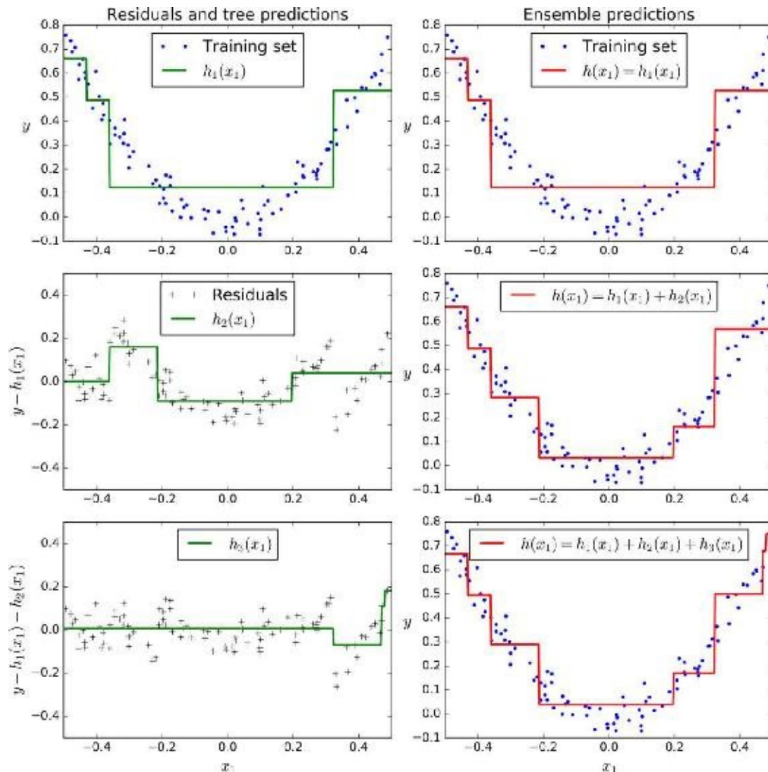
Figure 7-9. Gradient Boosting
