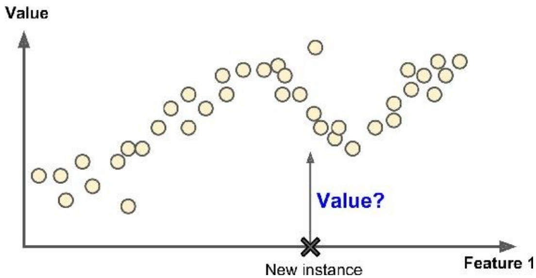
Figure 1-6. Regression
