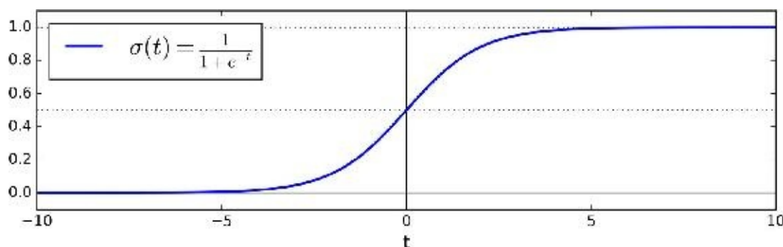
Figure 4-21. Logistic function
