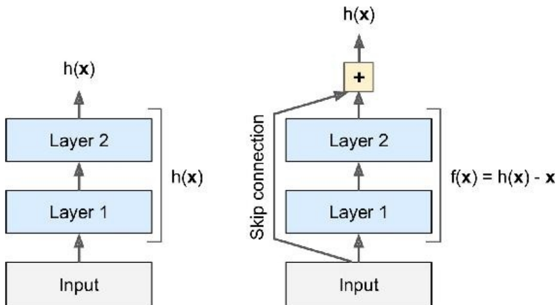
Figure 13-12. Residual learning
