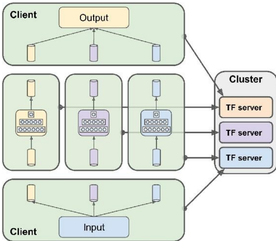
Figure 12-13. Between-graph replication
