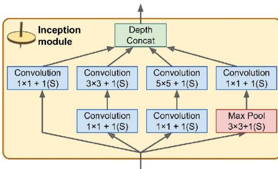
Figure 13-10. Inception module
