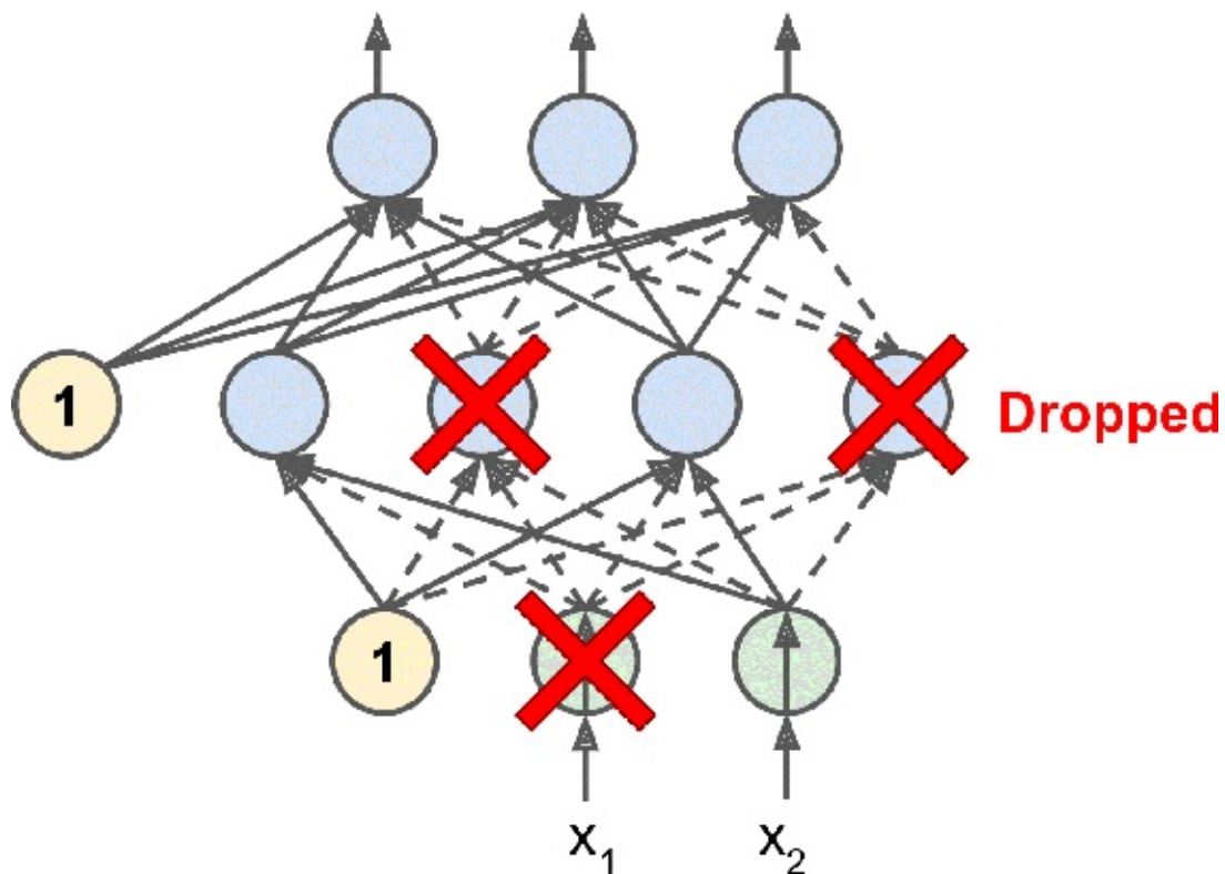
Figure 11-9. Dropout regularization
