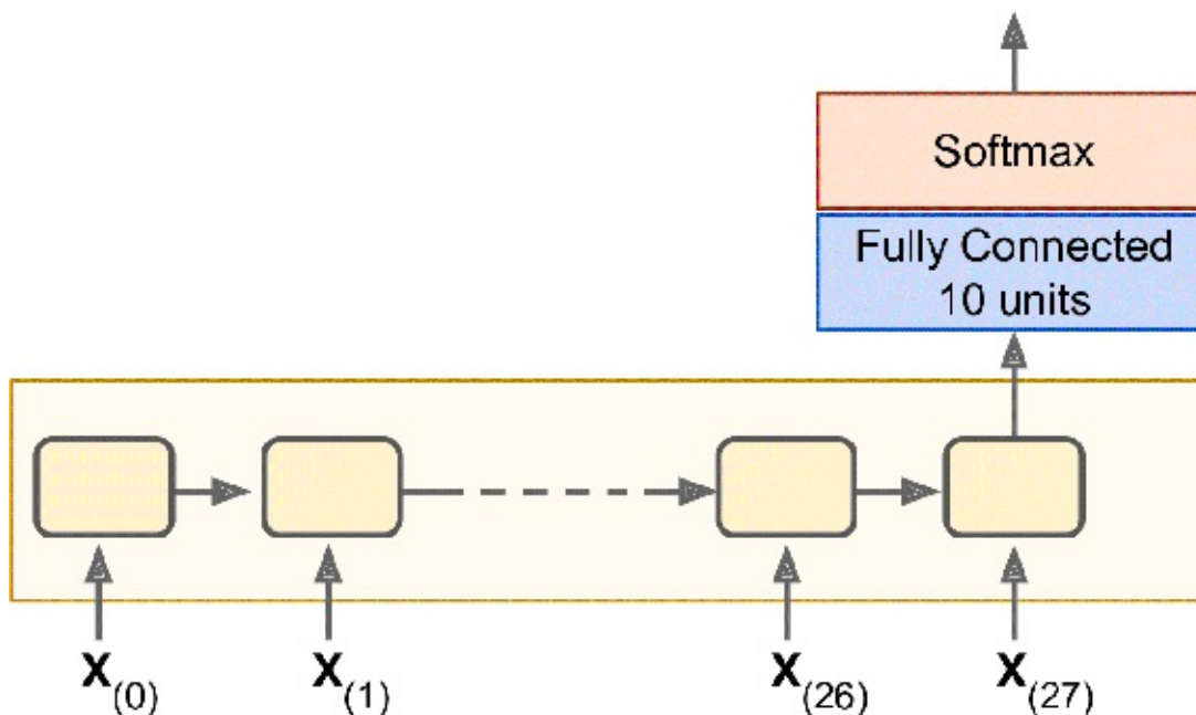
Figure 14-6. Sequence classifier
