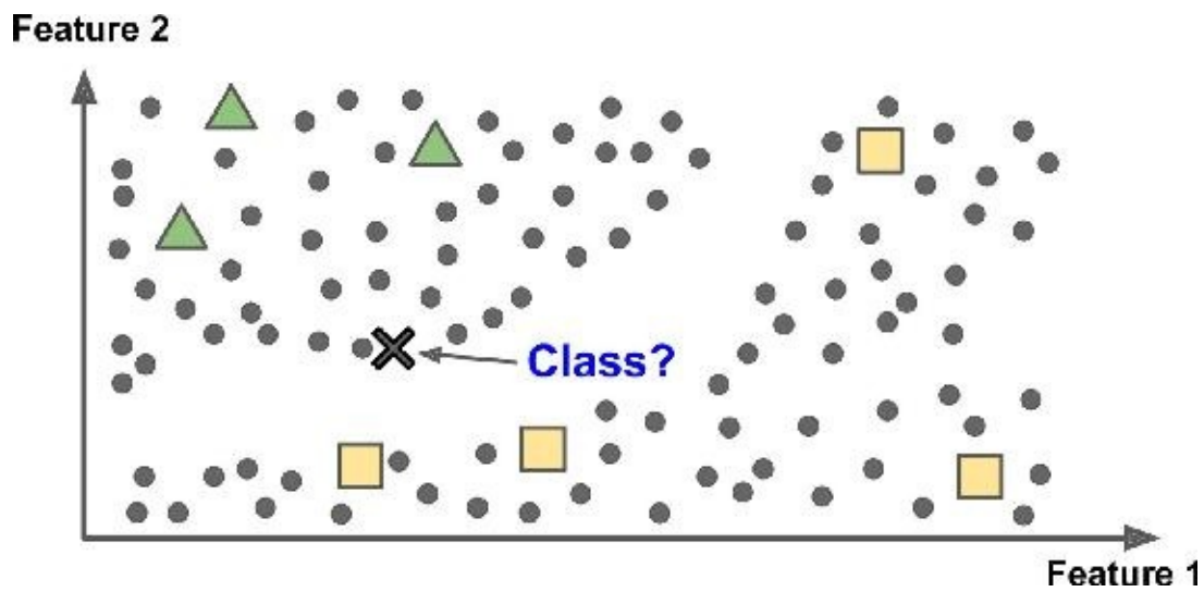
Figure 1-11. Semisupervised learning
